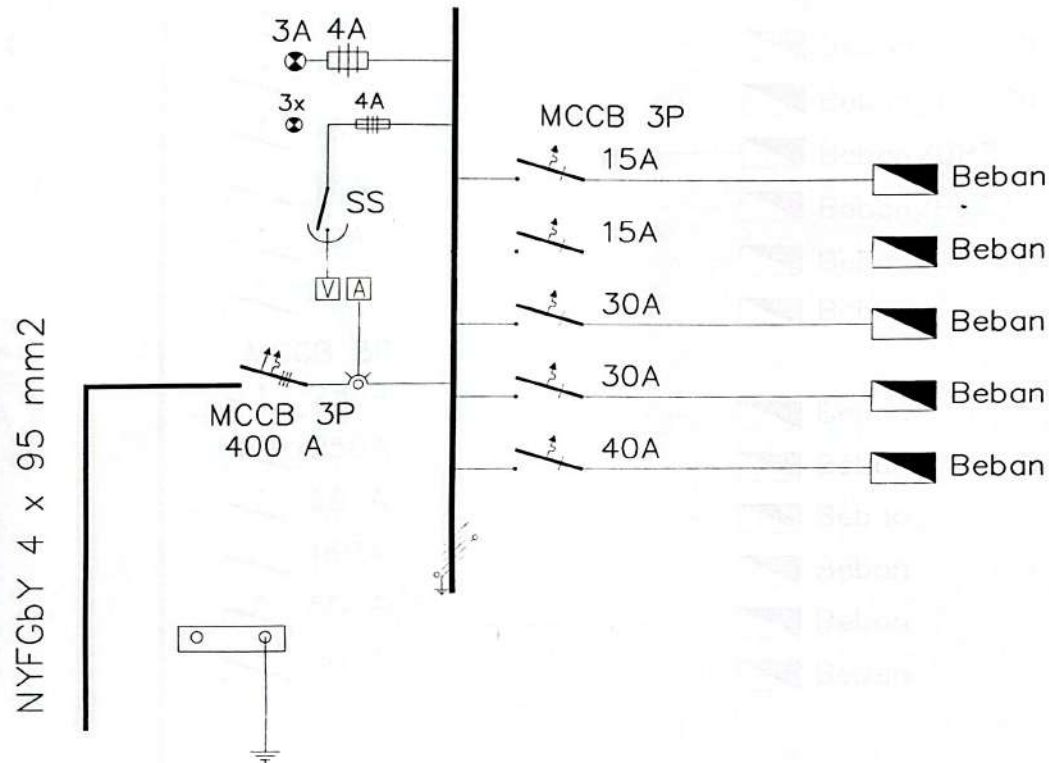
1 SINGLE LINE DIAGRAM PP. GEDUNG PASSENGER CAR(GD.I) MEP-EL SKALA : NTS
