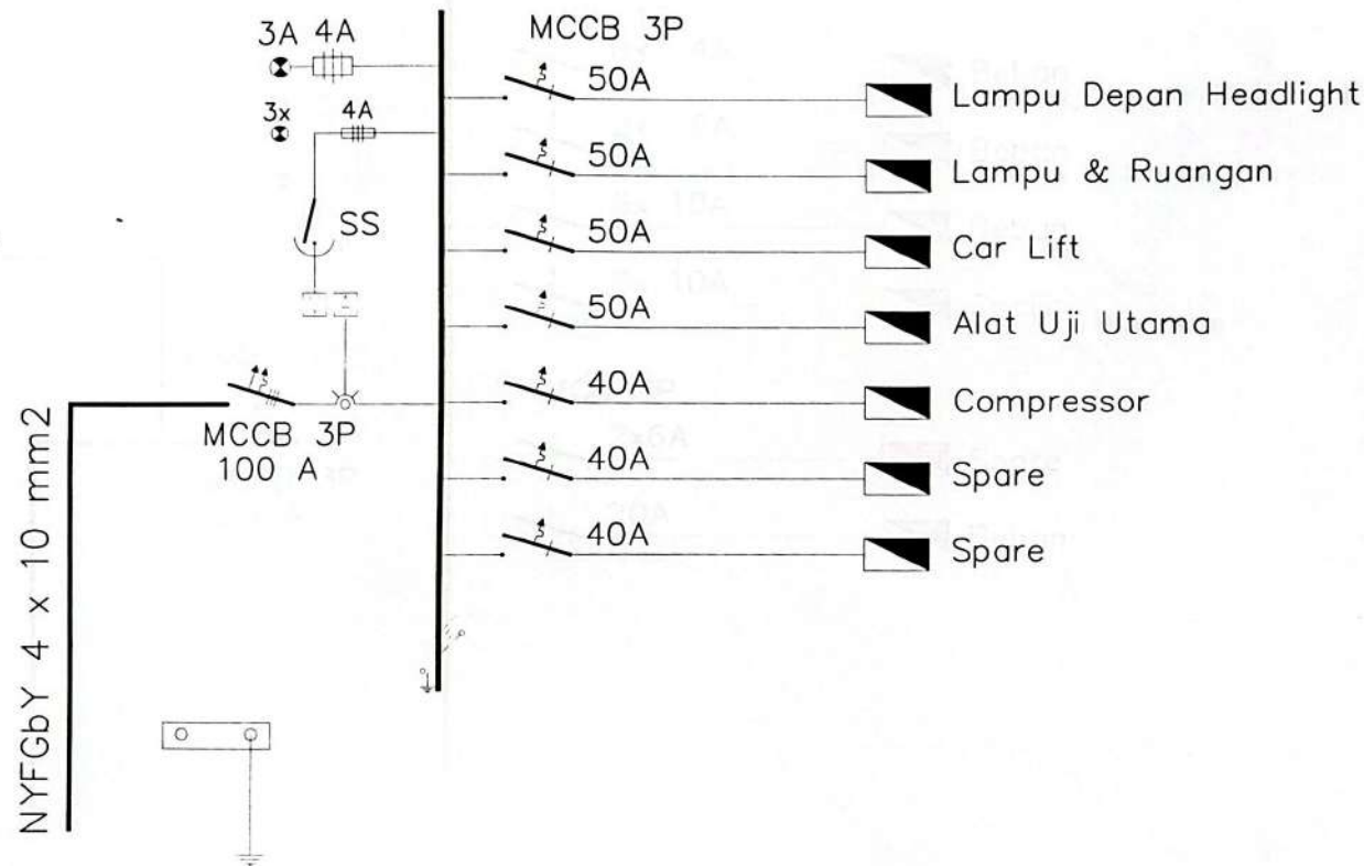
1 SINGLE LINE PP. GEDUNG ENGINE (GD.J) MEP-EL SKALA : NTS
