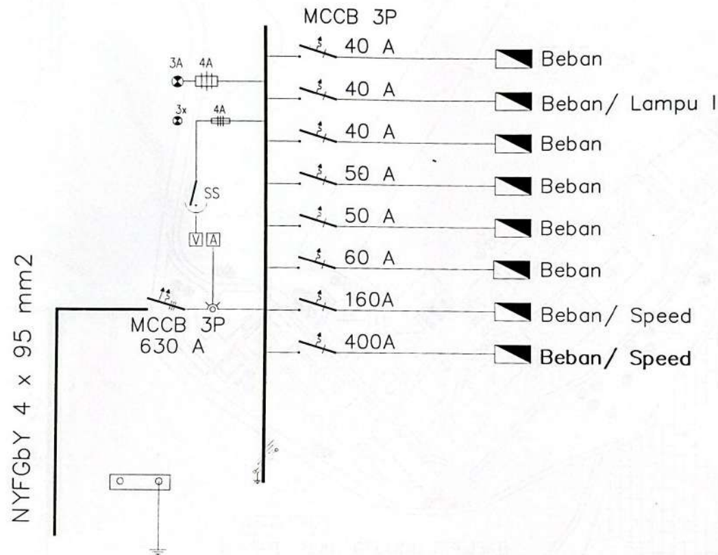
1 SINGLE LINE DIAGRAM PP. GEDUNG BRAKE (GD.K) MEP-EL SKALA : NTS
