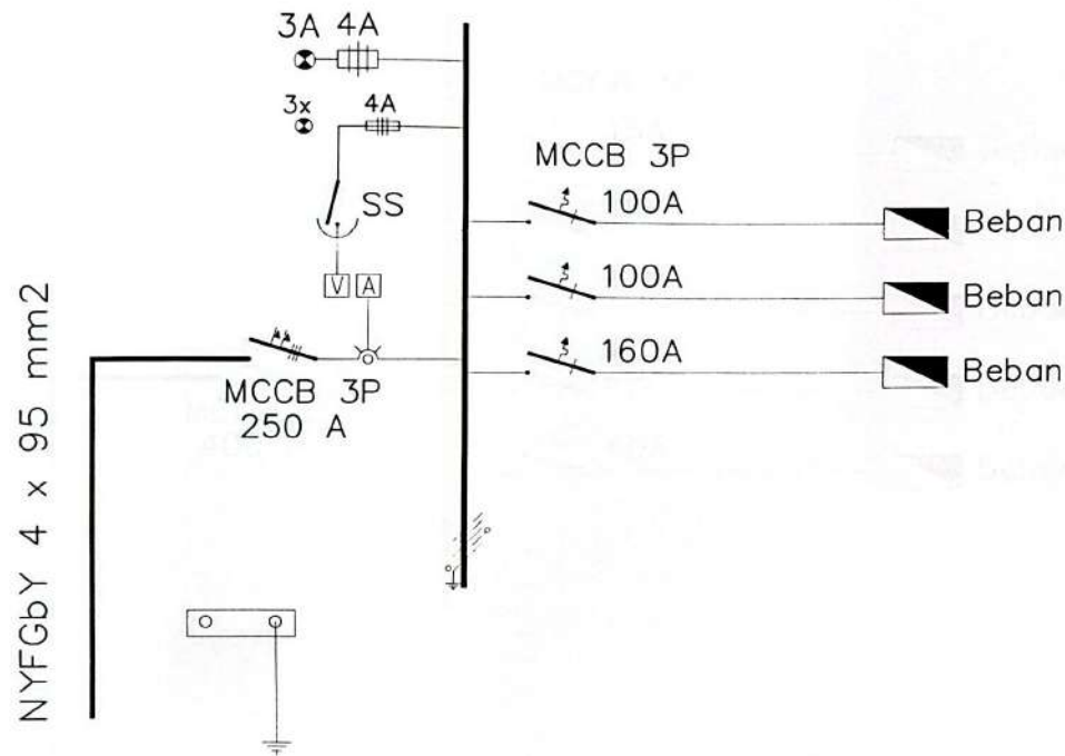
1 SINGLE LINE PP. KANTIN MEP-EL SKALA : NTS
