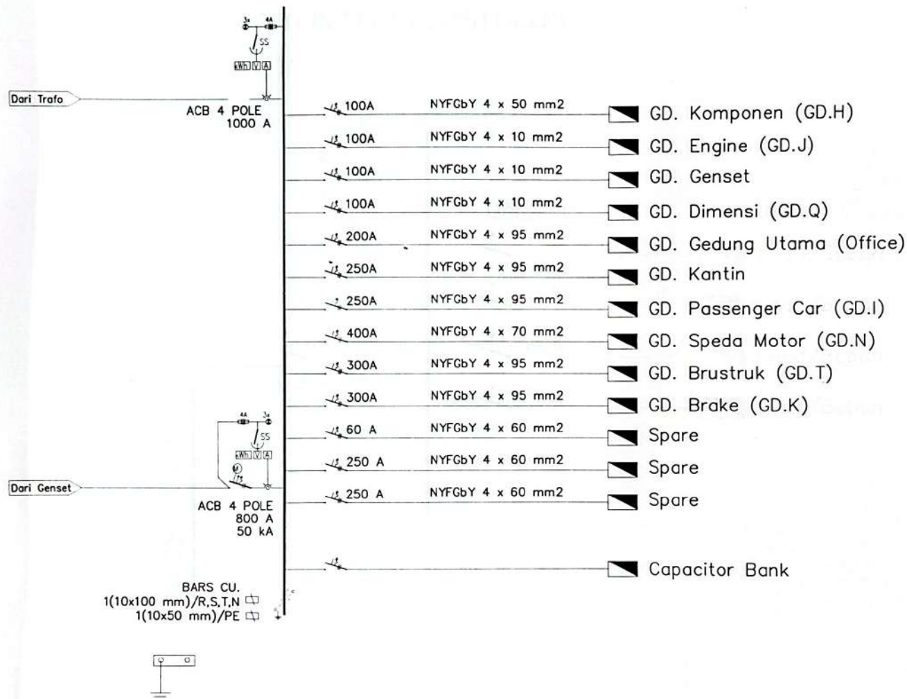
1 SINGLE LINE DIAGRAM LVMDP MEP-EL SKALA : NTS
