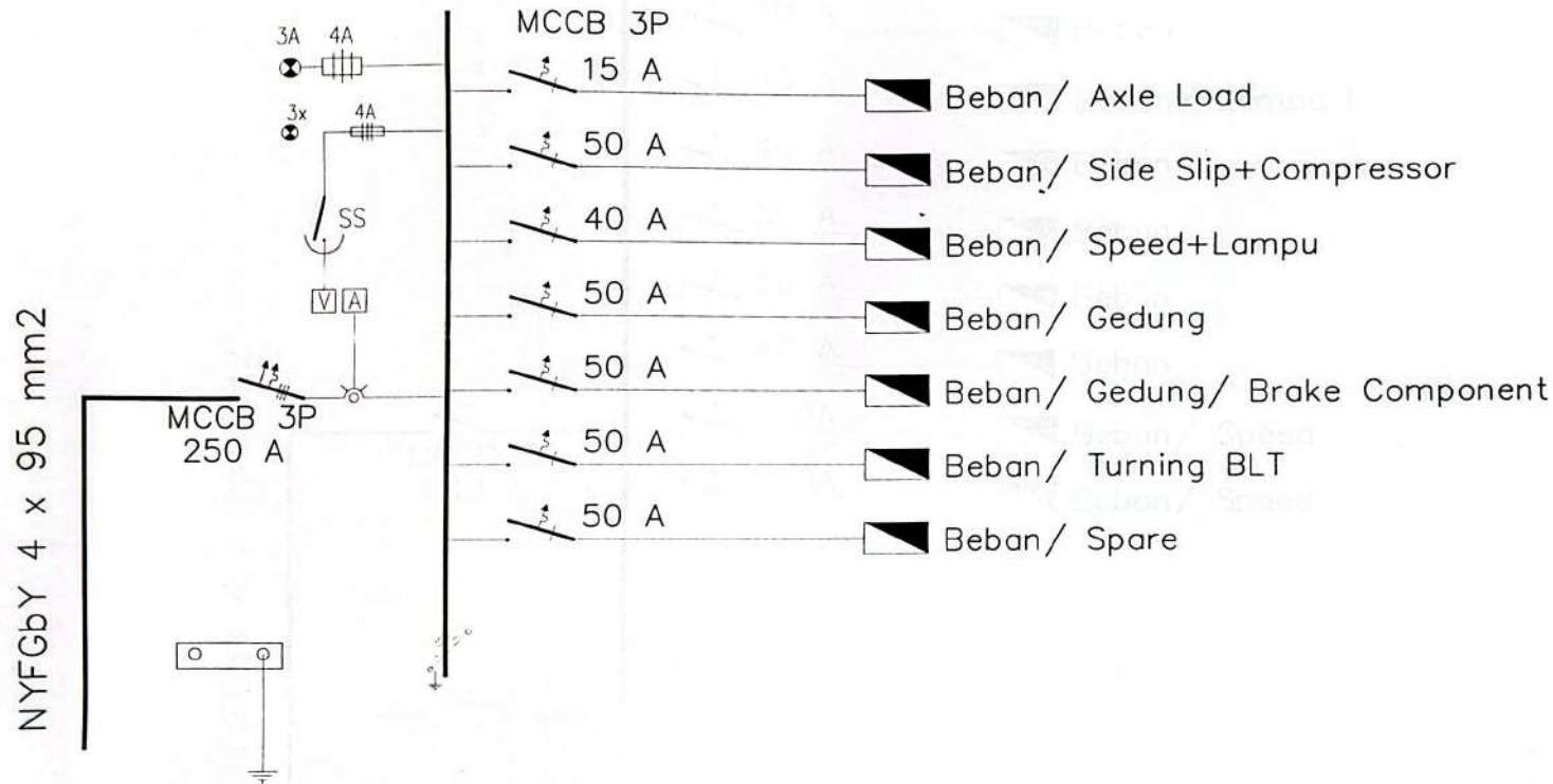
1 SINGLE LINE DIAGRAM PP. BUSTRUK (GD.T) MEP-EL SKALA : NTS
