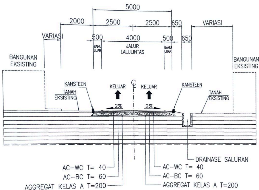
TYPICAL POTONGAN MELINTANG JALAN SEGMENT D SKALA 1 : 75
