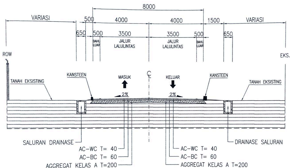
TYPICAL POTONGAN MELINTANG JALAN SEGMENT A SKALA 1 : 75
