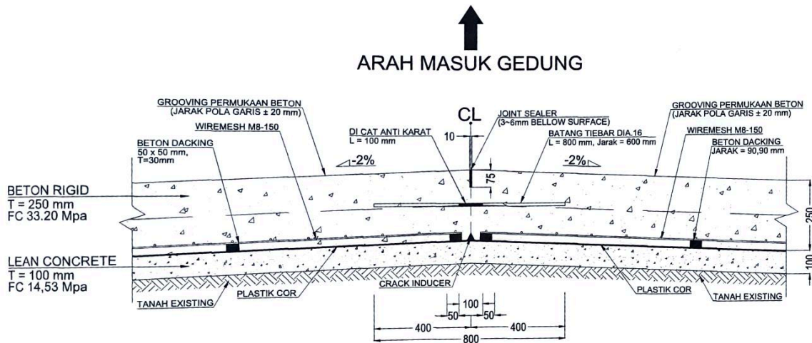
DETAIL JOINT MELINTANG TIEBAR SKALA 1:30
