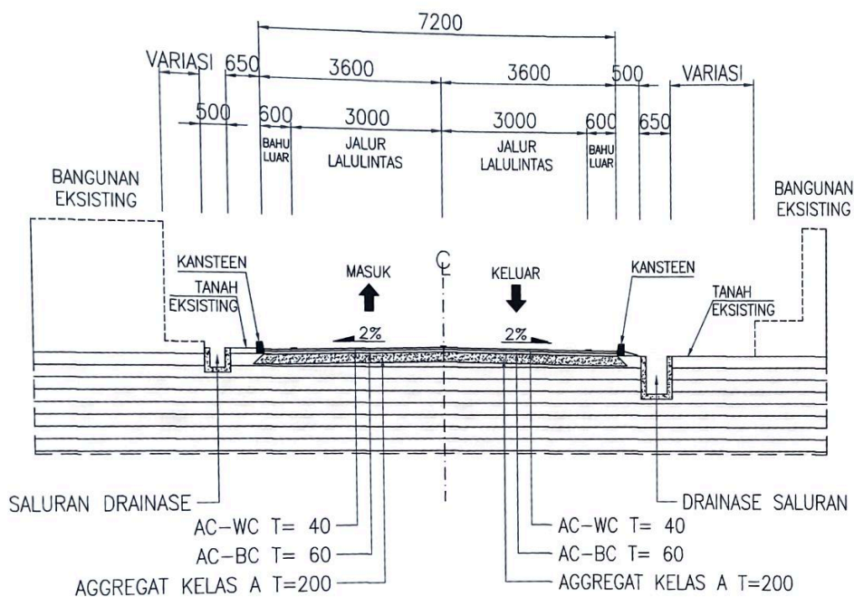
TYPICAL POTONGAN MELINTANG JALAN SEGMENT B SKALA 1 : 75
