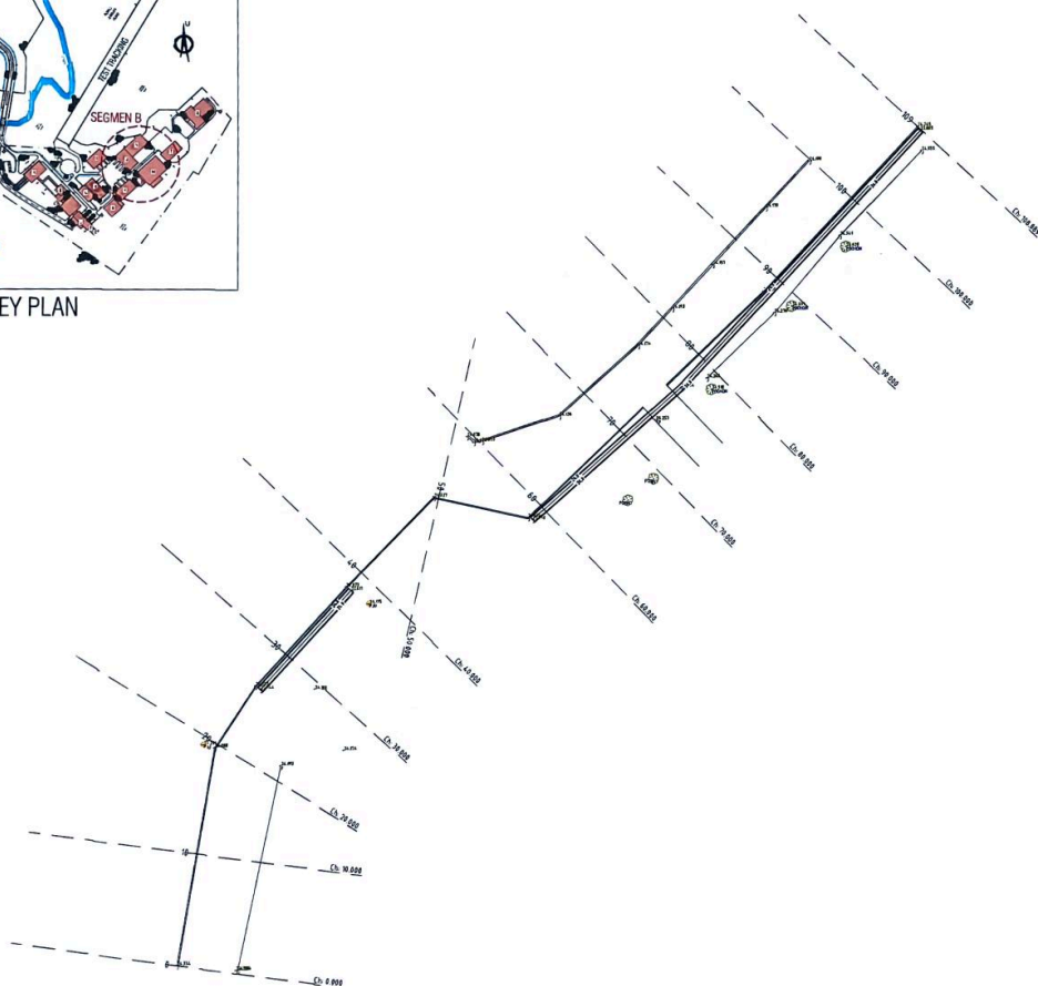
ALIGNMENT LAYOUT EXSISTING BPLJSKB SEGMENT B
