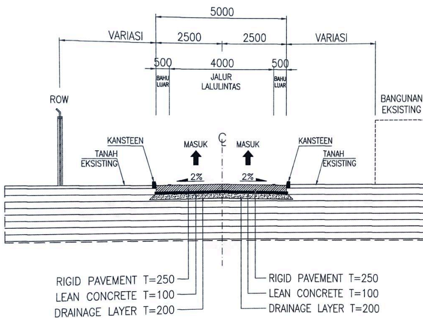
TYPICAL POTONGAN MELINTANG JALAN SEGMENT C SKALA 1 : 75
