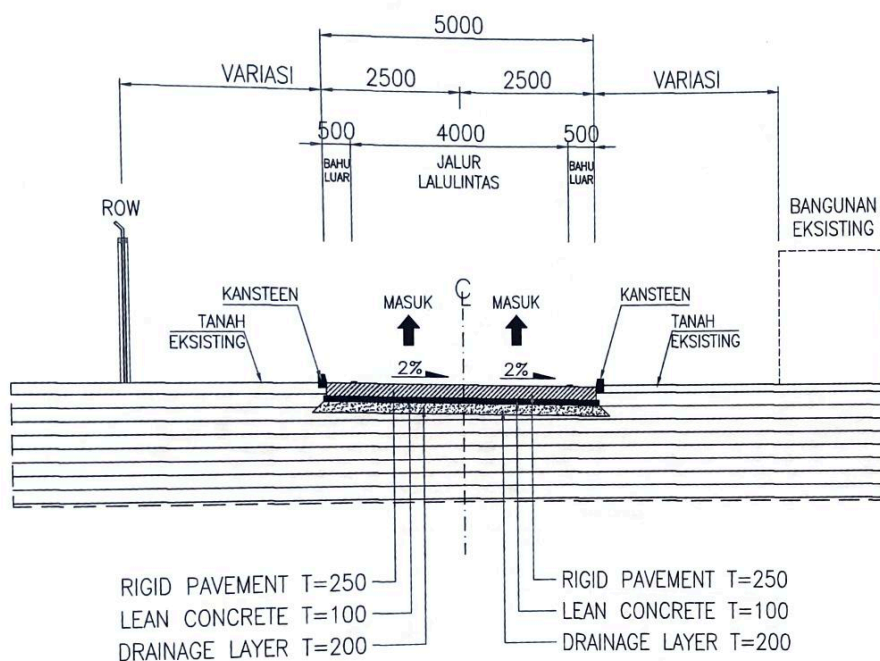
TYPICAL POTONGAN MELINTANG SUPERELEVASI JALAN SEGMENT C SKALA 1 : 75
